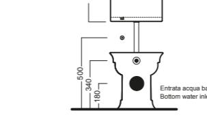
Entrata acqua bassa (sx) Bottom water inlet (left)
